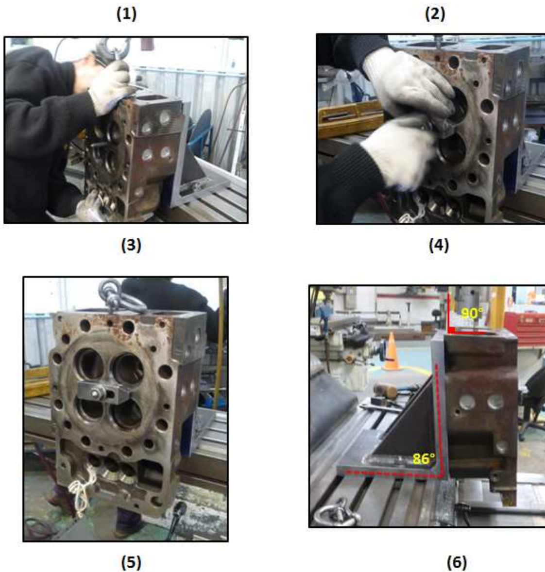
Picture 3. Steps to Tighten the head as cylinder
